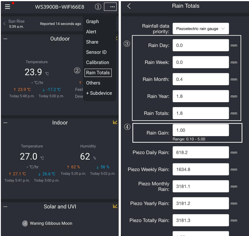
Figure 55: Rainfall Calibration
